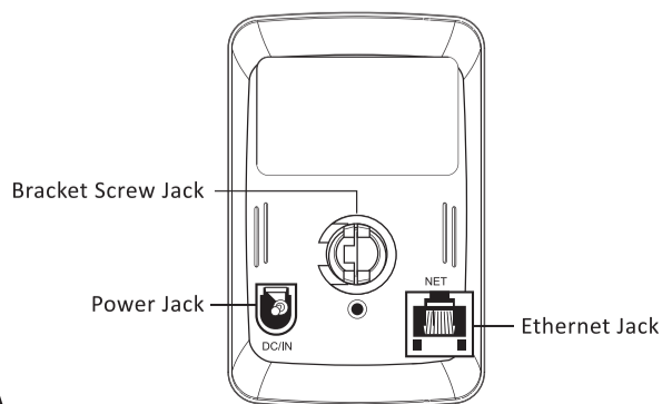
[ Back View ]
