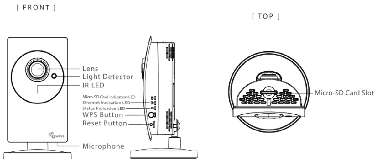
Figure 2-1: Major components in the front panel
